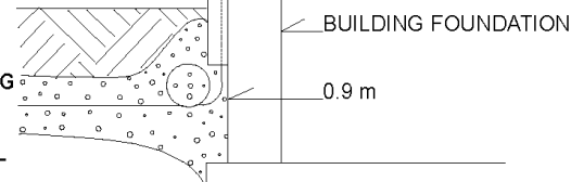
CABLE DETAIL IF NO METER SOCKET.
